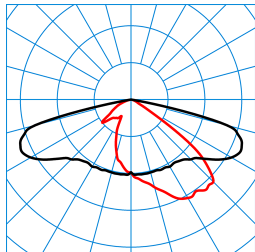
LIQ 70N-AB7L-SLR2/14500-727 12G1 ET (CLO initial value) TX778098 ■ C0 - C180 ■ C90 - C270 DIN 5040: A30 UTE: 1,00 E DLOR: 100 % ULOR: 0 % CEN Flux Code: 39 76 98 100 100
