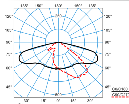
LIQ 70N-AB7L-LRA/75/82/91-722 10G1 ETDD (CLO initial value)
