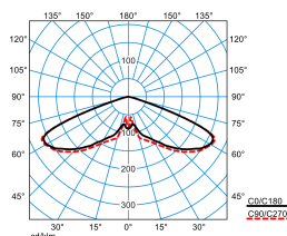
Publisca P1-RB6L/3200-740 4G1S ETDD (CLO initial value) TX300900
