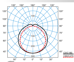
Deveo G3 12 DL 20-61/3ML-8MC ET PC +LV (stage 1)
