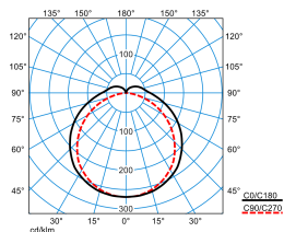
Deveo G3 12 DL 20-61/3ML-8MC ET PC +LV (stage 3)
