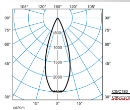
SNS QC3-WR1FL-14-930 1 20
