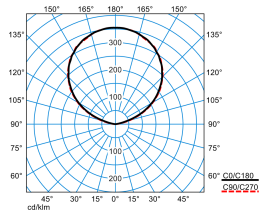
Parella H-LM 11500-830 03 (indirect) TX057128
