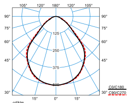
Parella H-LM 11500-830 03 (direct c90geo) TX057127
