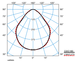
Parella H-LM 11500-830 03 (direct c270geo) TX057126
