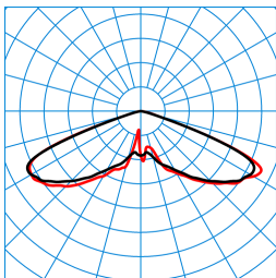
Publisca P2-RB6L-LR/2200-730 3G1S ET (CLO initial value) TX300183 ■ C0 - C180 ■ C90 - C270 DIN 5040: A20 UTE: 1,00 J DLOR: 100 % ULOR: 0 % CEN Flux Code: 20 57 98 100 100
