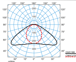
Nextrema G3 XB40-840 ETDD+HFSX LV TWP PC
