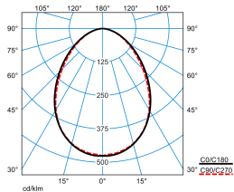
SFLOW C2-L MRWD LED4000-830 ETDD 01 TX721368
