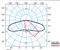
LIQ 50N-AB2L-LR/220/260/320-740 4G1 ET (CLO end value) TX777525
