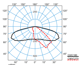
LIQ 50N-AB2L-LR/220/260/320-740 4G1 ET (CLO end value)
