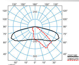
LIQ 50N-AB2L-LR/220/260/320-740 4G1 ET (CLO initial value)
