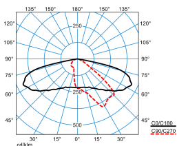
LIQ 50N-AB2L-LR/220/260/320-740 4G1 ET (CLO initial value) TX777529
