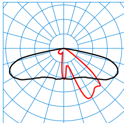
Publisca P2-AB2L/1200-740 2G1S ETDD (CLO initial value) TX301041 ■ C0 - C180 ■ C90 - C270 DIN 5040: A30 UTE: 1,00 G DLOR: 100 % ULOR: 0 % CEN Flux Code: 34 70 96 100 100
