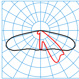
Publisca P2-AB2L/1200-740 2G1S ETDD (CLO end value) TX301415 ■ C0 - C180 ■ C90 - C270 DIN 5040: A30 UTE: 1,00 G DLOR: 100 % ULOR: 0 % CEN Flux Code: 34 70 96 100 100
