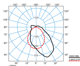
TugraHE 6 PAW 22-36/16ML-830 ET PC 23 (stage 3)
