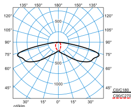
LIQ 50-SB3L/1000-730 2G1S ET TX777686 DIN 5040: A30 UTE: 1,00 l DLOR: 100 % ULOR: 0 % CEN Flux Code: 33 67 93 100 100
