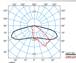
LIQ 50N-AB2L-LR/1650-740 2G1 ET (CLO initial value)
