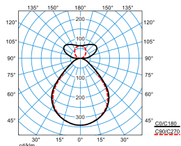
Opendo H1-L PW19 20-53/6/ML-830 ET 03 (3200lm)
