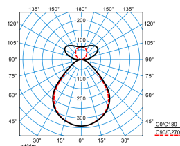
Opendo H1-L PW19 20-53/6/ML-830 ET 03 (5000lm)
