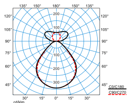
Opendo H1-L PW19 20-53/6/ML-830 ET 03 (2900lm)
