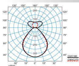
Opendo H1-L PW19 20-53/6/ML-830 ET 03 (1900lm)
