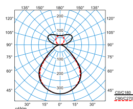
Opendo H1-L PW19 20-53/6/ML-830 ET 03 (4000lm)
