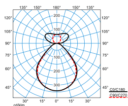
Opendo H1-L PW19 20-53/6/ML-830 ET 03 (2100lm)
