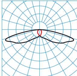
LIQ 50N-SB3L-LR/1350-740 2G1 ET (CLO end value) TX776237 ■ C0 - C180 ■ C90 - C270 DIN 5040: A30 UTE: 1,00 l DLOR: 100 % ULOR: 0 % CEN Flux Code: 31 64 92 100 100
