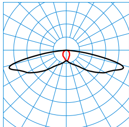
LIQ 50N-SB3L-LR/1350-740 2G1 ET (CLO initial value) TX776238 ■ C0 - C180 ■ C90 - C270 DIN 5040: A30 UTE: 1,00 l DLOR: 100 % ULOR: 0 % CEN Flux Code: 31 64 92 100 100
