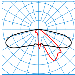
Publisca P2-AB2L/2600-730 3G1S ETDD (CLO initial value) TX301905 ■ C0 - C180 ■ C90 - C270 DIN 5040: A30 UTE: 1,00 l DLOR: 100 % ULOR: 0 % CEN Flux Code: 34 71 96 100 100
