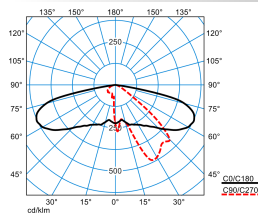
Publisca P2-AB2L/2600-730 3G1S ETDD (CLO initial value)
