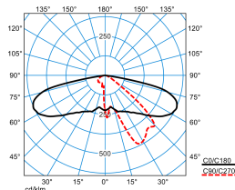
Publisca P2-AB2L/2600-730 3G1S ETDD (CLO end value)
