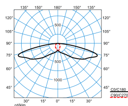
LIQ 50N-SB3L-LRA/1500-727 2G1 ETDD (CLO end value)
