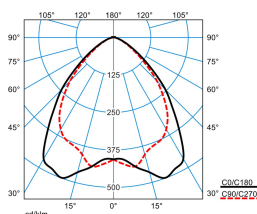
ELINE LW40-110 ML 840 L150 2 50
