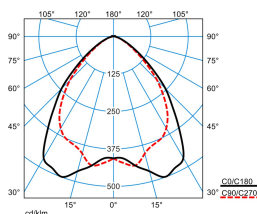
ELINE LW40-110 ML 840 L150 4 50
