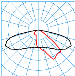
LIQ 50N-AB2L-LRA/51/56/62-740 6G1 ETDD (CLO end value) TX775880
