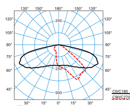
LIQ 50N-AB2L-LRA/51/56/62-740 6G1 ETDD (CLO end value)
