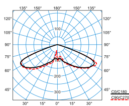
Publisca P1-RB6L-LR/2000-740 3G1S ET (CLO initial value) TX301587 DIN 5040: A20 UTE: 1,00 J DLOR: 100 % ULOR: 0 % CEN Flux Code: 20 57 98 100 100
