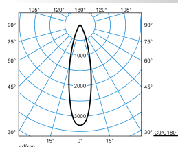
OsidoRW-RE3L-10-830-ETDD-GS26
