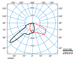
LIQ 50N-FL1L/5600-730 6G1 ET (CLO end value)
