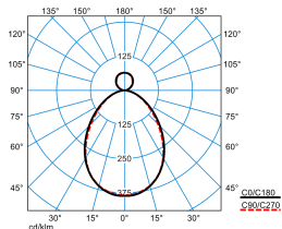
SFlow H2-L MRWD LED5400-840 ETDD EB3 03
