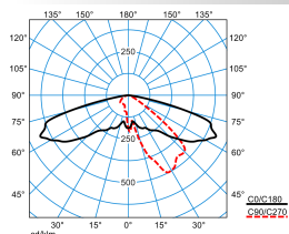
Publisca P1W-AB2L-LRA/3200-740 4G1S
