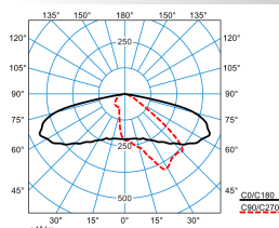
LIQ 50N-AB2L-LR/2200-740 4G1 ET (CLO initial value)
