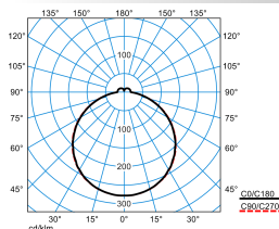
Olisq QWD2 DW 35-8TW ETBLE +CAS IP54 (DWW)
