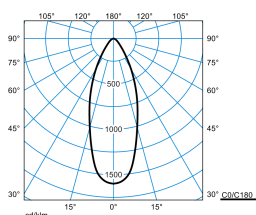
Amatris QC1 SRRFL 4-9MC ET 05 2KIT + PC IP54 (stage 2)
