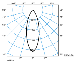
Amatris QC1 SRRFL 4-9MC ET 05 2KIT + HC-19 05 (stage 3)
