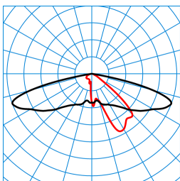
Publisca P1W-AB2L-LR/2600-730 3G1S ET (CLO initial value) TX300299 ■ C0 - C180 ■ C90 - C270 DIN 5040: A30 UTE: 1,00 l DLOR: 100 % ULOR: 0 % CEN Flux Code: 32 69 96 100 100 0 33 67 0
