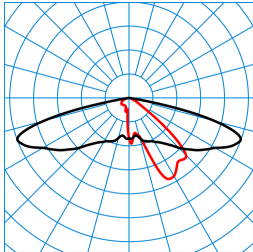
Publisca P1W-AB2L-LR/2600-730 3G1S TX053483 ■ C0 - C180 ■ C90 - C270 DIN 5040: A30 UTE: 1,00 l DLOR: 100 % ULOR: 0 % CEN Flux Code: 32 69 96 100 100 0 33 67 0
