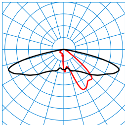
Publisca P1W-AB2L-LR/2600-730 3G1S ET (CLO end value) TX301397 ■ C0 - C180 ■ C90 - C270 DIN 5040: A30 UTE: 1,00 l DLOR: 100 % ULOR: 0 % CEN Flux Code: 32 69 96 100 100 0 33 67 0
