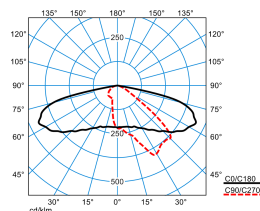
LIQ 50N-AB2L-LR/4600-727 6G1 ET (CLO end value)
