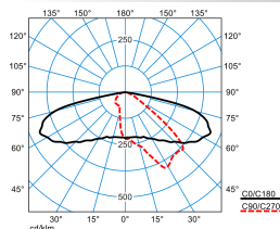
LIQ 50N-AB2L-LR/4600-727 6G1 ET (CLO initial value)
