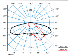
LIQ 50N-AB2L-LR/4600-727 6G1 ET (CLO initial value)
