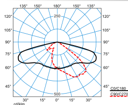
LIQ 70N-AB7L-LR/6800-740 8G1 ET(CLO initial value)
