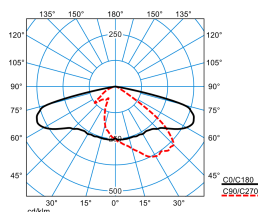
LIQ 70N-AB7L-LR/6800-740 8G1 ET(CLO end value)
