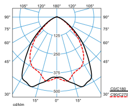
ELINE LW40-110 ML 840 L150 4 20
