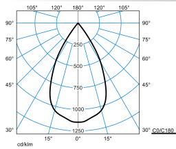
E-Line PRO 78 BV G2 RF-VFL 50-830 M33 ETBLE 03 Blank
