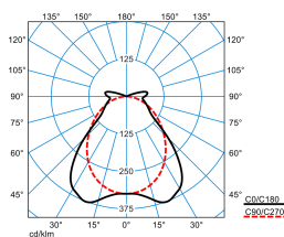
ArX12PW30-80ML840ET+UPG PC (stage 5)
