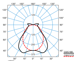
ArX12PW30-80ML840ET+UPG PC (stage 2)
