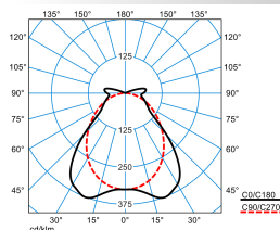
ArX12PW30-80ML840ET+UPG PC (stage 1)
