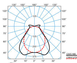
ArX12PW30-80ML840ET+UPG PC (stage 4)
