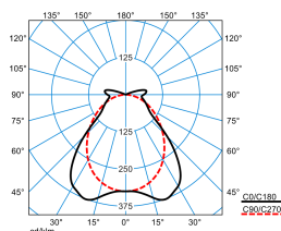
ArX12PW30-80ML840ET+UPG PC (stage 3)
