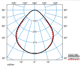
Opendo D1-L PW19 20-36/4/ML-840 ET 03 (2000lm) TX376521
