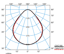
Opendo D1-L PW19 20-36/4/ML-840 ET 03 (3600lm) TX376524
