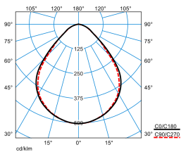
Opendo D1-L PW19 20-36/4/ML-840 ET 03 (2500lm) TX376522
