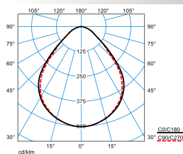
Opendo D1-L PW19 20-36/4/ML-840 ET 03 (2000lm)
