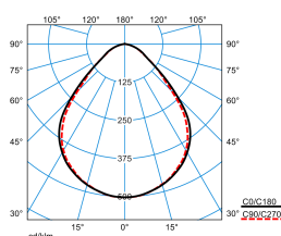
Opendo D1-L PW19 20-36/4/ML-840 ET 03 (3600lm)
