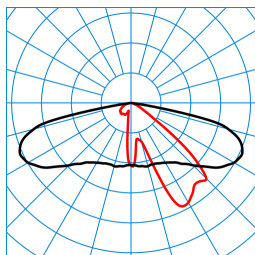
Publisca P2-AB2L/1100-730 2G1S ETDD (CLO initial value) TX301612 ■ C0 - C180 ■ C90 - C270 DIN 5040: A30 UTE: 1,00 G DLOR: 100 % ULOR: 0 % CEN Flux Code: 34 70 96 100 100
