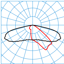
LIQ 50N-AB2L-SLR2/4200-730 4G1 ET (CLO initial value) TX777263
