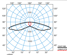
LIQ 50N-SB3L-LR/1650-727 2G1 ET (CLO end value)
