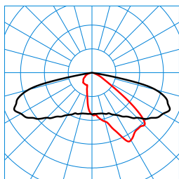
LIQ 50N-AB2L-LR/510/560/620-730 6G1 ET (CLO initial value) TX775770
