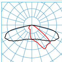
LIQ 50N-AB2L-LR/510/560/620-730 6G1 ET (CLO end value) TX775769
