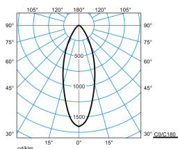
Amatris RC2 SRRFL 8-9MC ET 05 2KIT + PC IP54 (stage 1)
