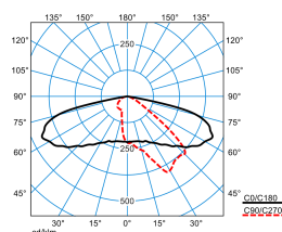
LIQ 50N-AB2L-SLR2/2200-740 2G1 ET (CLO end value)
