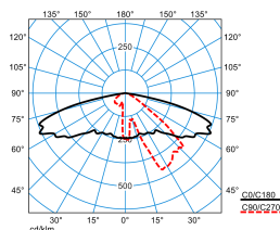
Publisca P1W-AB2L/1200-730 2G1S
