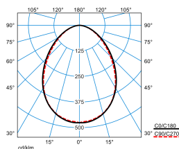
SFlow C1-L MRWD LED3200-840 ET 01 TX721350
