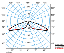
CS 19 100-RB6L/3800-740 4G1S ETDD (CLO initial value) TX300114
