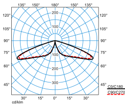
CS 19 100-RB6L/3800-740 4G1S ETDD (CLO end value) TX300113
