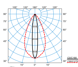
Altigo G2 C 60 SE6L/800-830 1G1P + VE IP66 24V DC 60W
