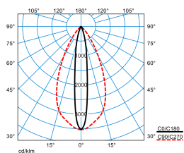
Altigo G2 C 60 SE6L/800-830 1G1P + VE IP66 24V DC 130W
