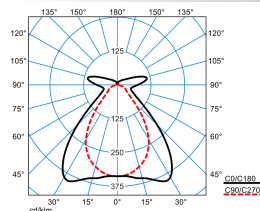
TugraHE+ 12 PW19 38-840 ETDD 01
