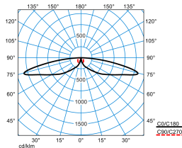
CS 19 100-SB3L-SLR1/2200-727 4G1S ET (CLO end value)
