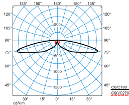
CS 19 100-SB3L-SLR1/2200-727 4G1S ET (CLO initial value)
