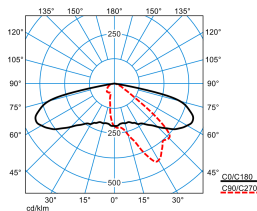
Cuvia60-AB2L12LR-S2-135-730-ET-CAE-26 (CLO initial value) TX565097
