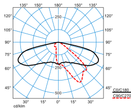
Cuvia60-AB2L12LR-S2-135-730-ET-CAE-26 (CLO end value) TX565096
