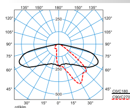
Cuvia60-AB2L12S2-135-727-ET-CAB-26 (CLO initial value)
