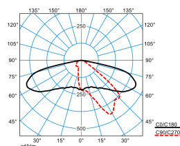
Cuvia60-AB2L12S2-135-727-ET-CAB-26 (CLO end value)
