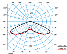
Publisca P2-RB6L/4600-730 6G1S ETDD (CLO end value)
