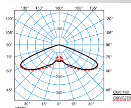
Publisca P2-RB6L/4600-730 6G1S ETDD (CLO initial value)
