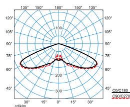
Publisca P2-RB6L/4600-730 6G1S
